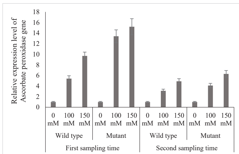
Figure 9. Relative expression of ascorbate peroxidase gene under different concentrations of salt stress in wild and mutant rice cultivars.
