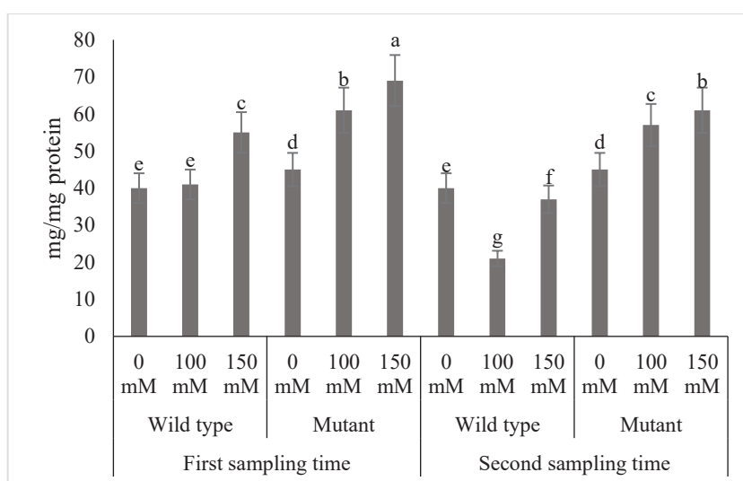
Figure 3. Catalase levels in wild and mutant rice genotypes under salt stress (LSD test, p \leq 0.05 ). Means with the same letter are not significantly different.
