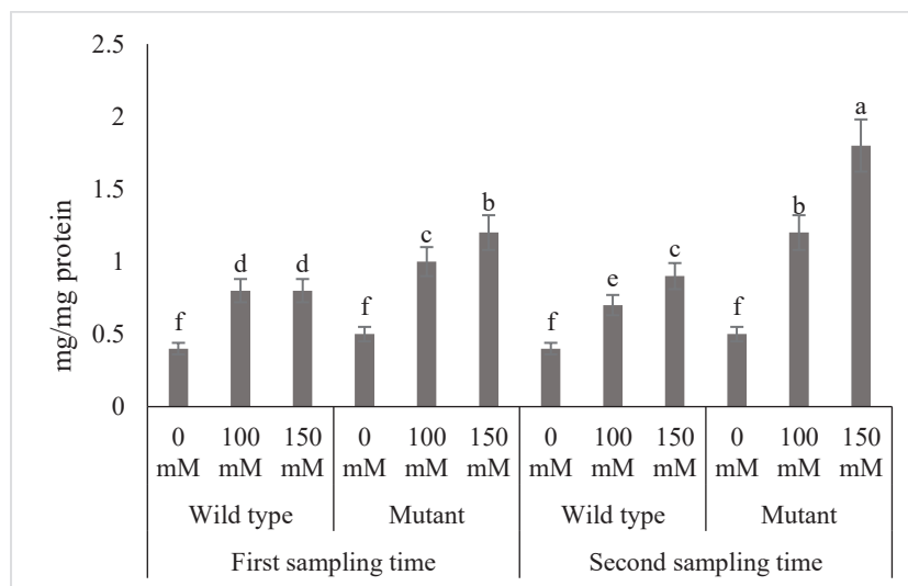
Figure 4. Ascorbate peroxidase levels in wild and mutant rice genotypes under salt stress (LSD test, p \leq 0.05 ). Means with the same letter are not significantly different.
