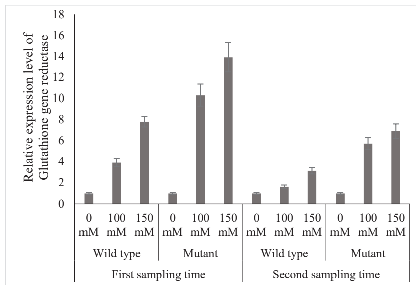
Figure 8. Relative expression of glutathione reductase gene under different concentrations of salt stress in wild and mutant rice cultivars.
