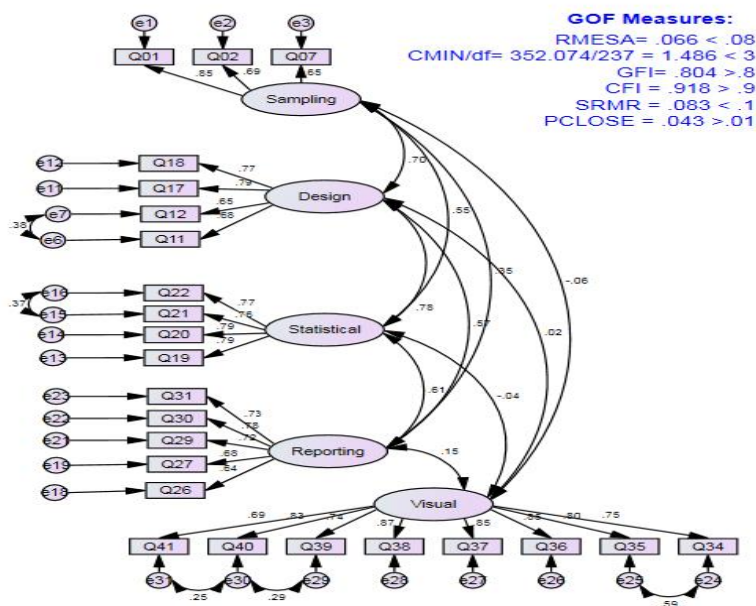
Standardized Estimates and GOF Values for the Modified Questionnaire
