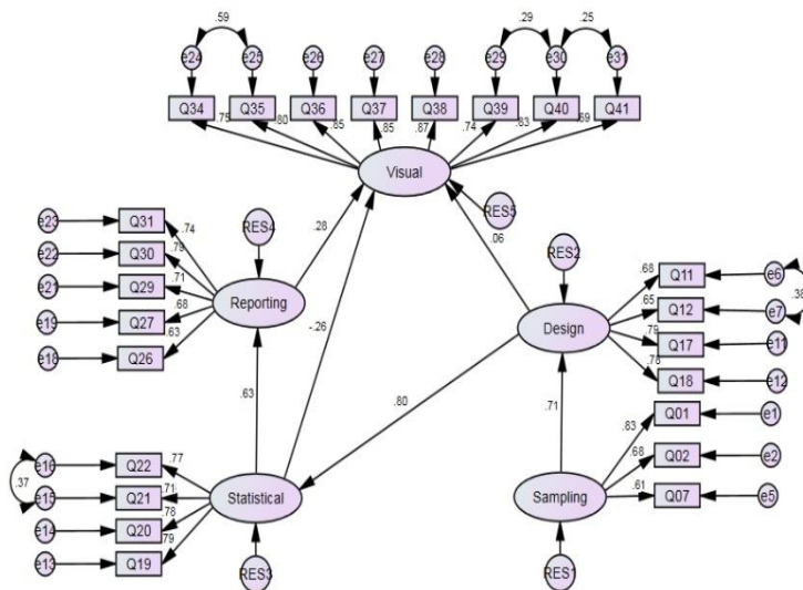
Standardized Estimates of the Structural Model
